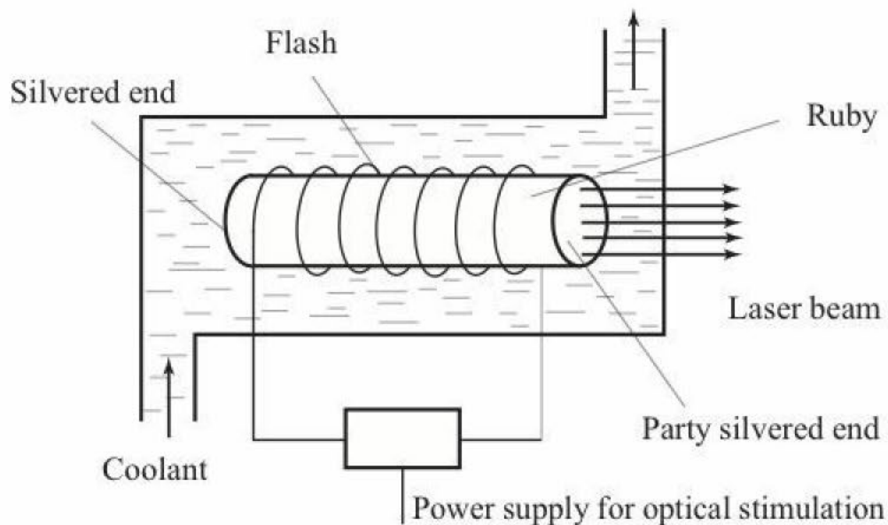
Diagram of a simple ruby laser
